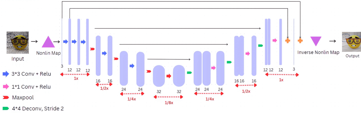
Denoising Model
